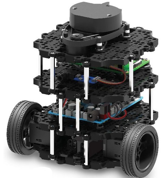
TurtleBot3 Burger
